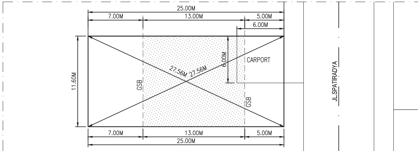
DENAH UNIT HUNIAN JL.SPATIRADYA NO. 28 SKALA 1 : 300
